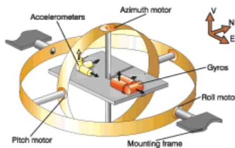
Figure 3.2. Schematic diagram of INS mechanism
