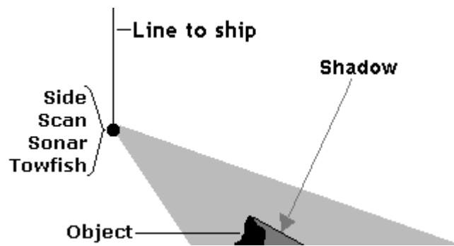
Figure 4.5. Sound way of side scan sonar
