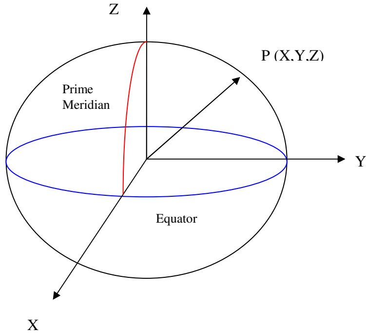
Figure 5.7. Earth centered earth fixed X, Y, Z coordinates
