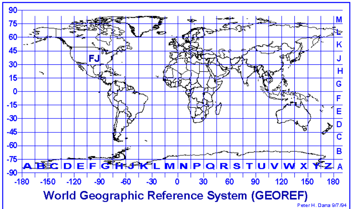
Figure 5.11. World geographic reference system
