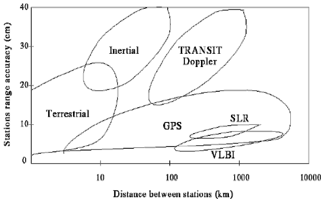
Figure 3.10. Stations range accuracy
