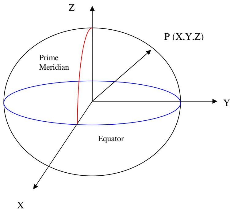
Figure 5.5. Equator and prime meridian
