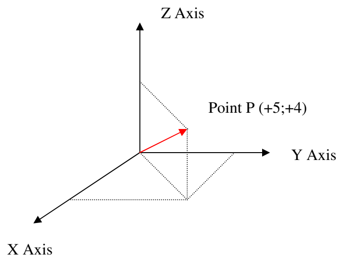
Figure 5.2. Three-dimensional cartesian coordinates
