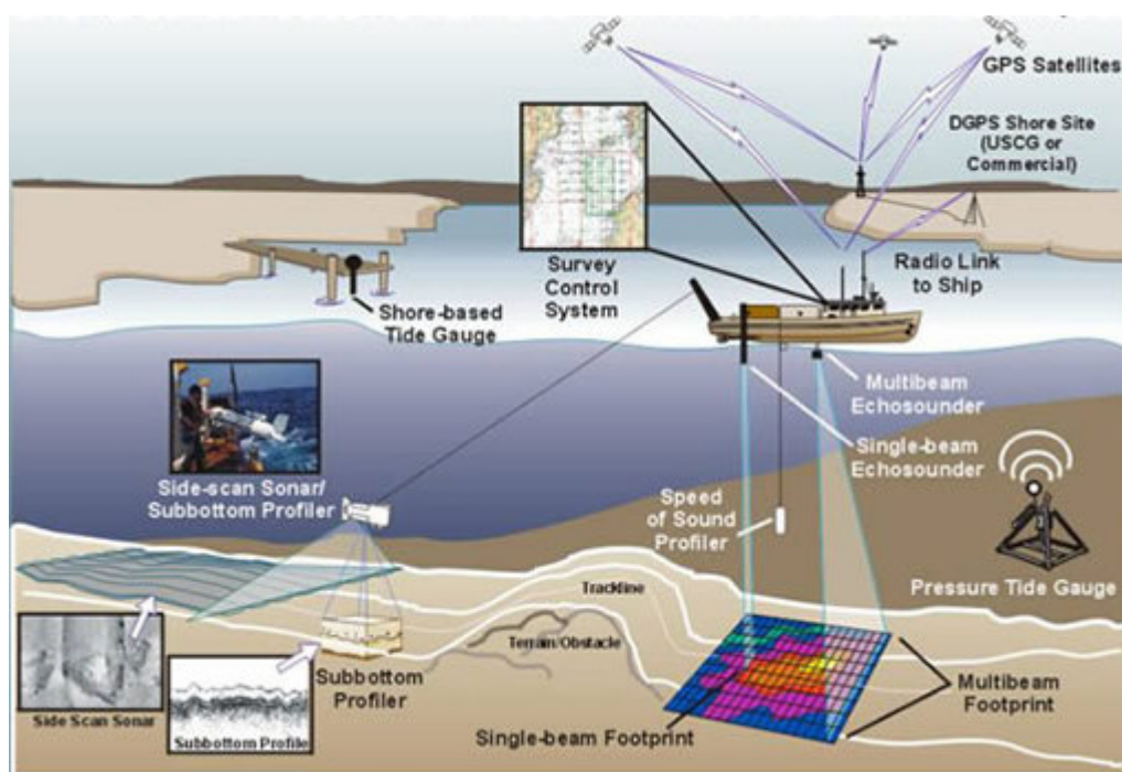
Figure 4.6. Acoustic seafloor characterization techniques
