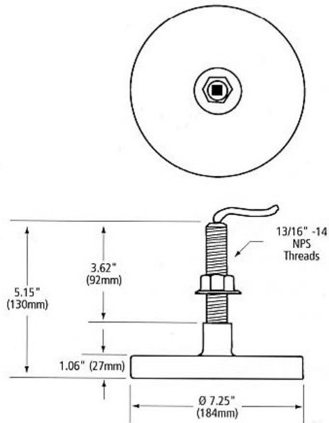
Figure 6.7. Dimensions of transducer's parts
