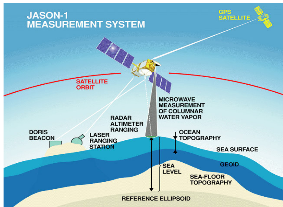
Figure 3.7. Jason-1 measurement system
