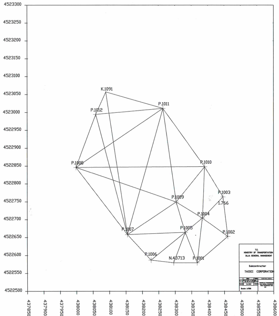
Figure 6.3. Primary and secondary control points of D.L.H. harbor
