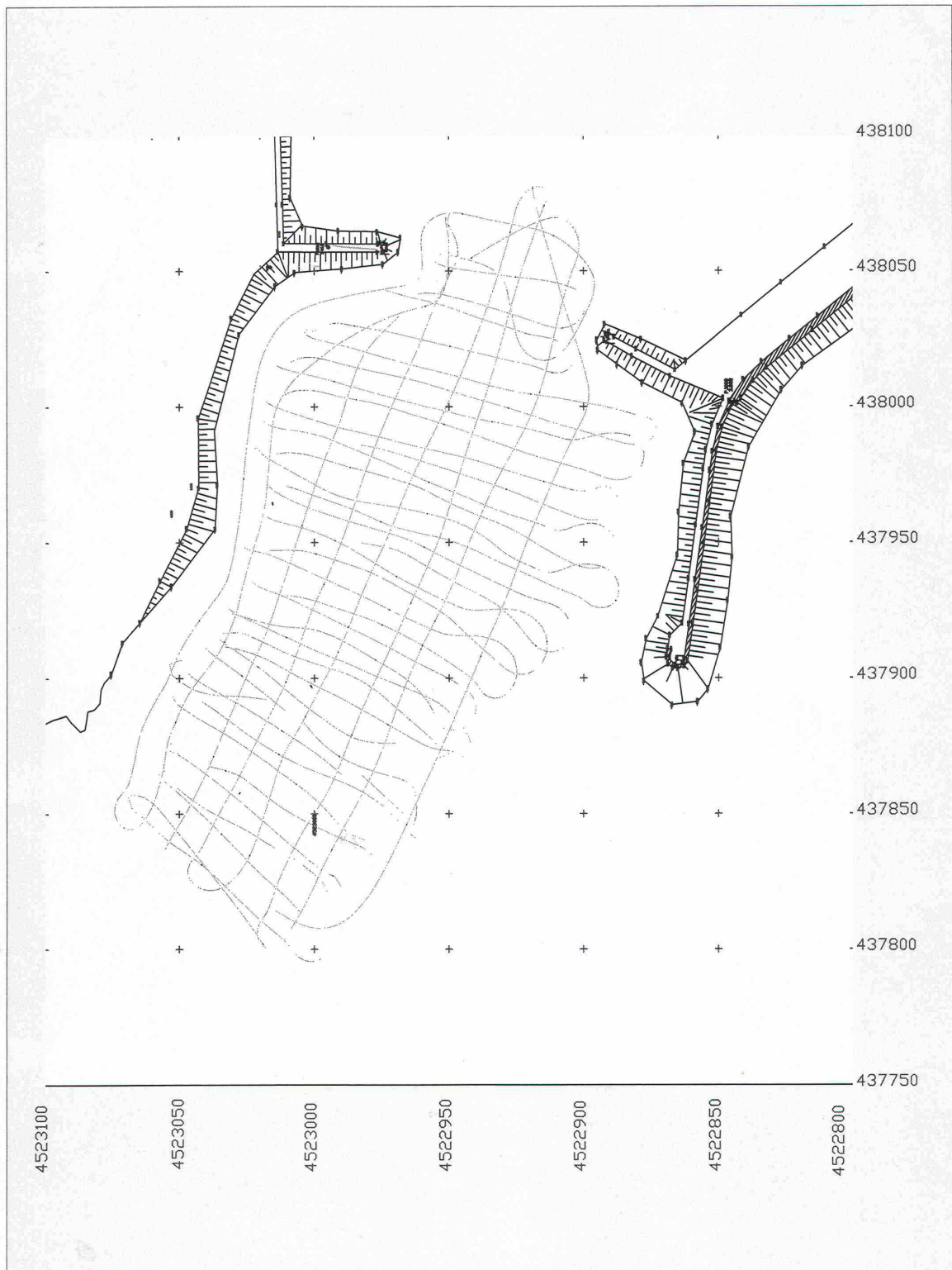
Figure 6.8. Bathymetric survey lines
