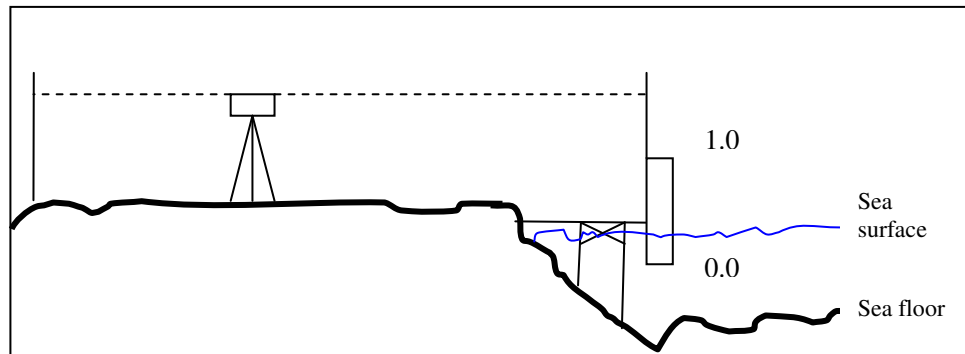
Figure 6.5. Tide gauge system
