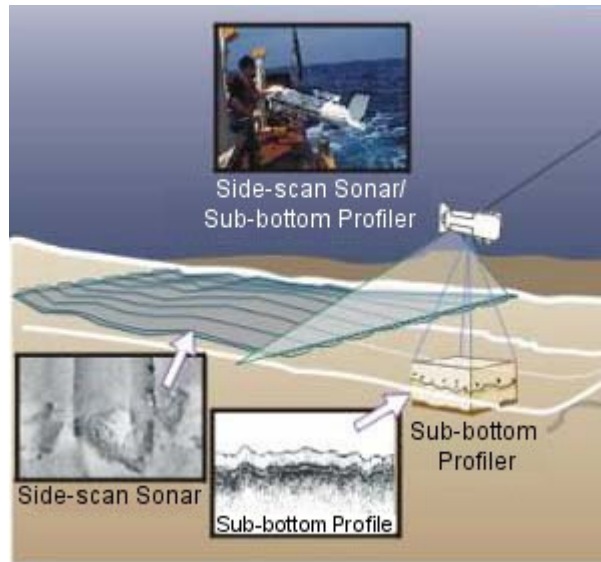
Figure 4.7. Sub-bottom profiler
