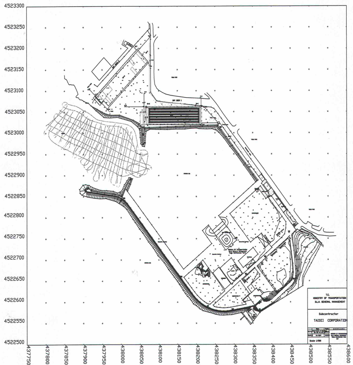
Figure 6.9. Bathymetric survey lines in D.L.H. harbor
