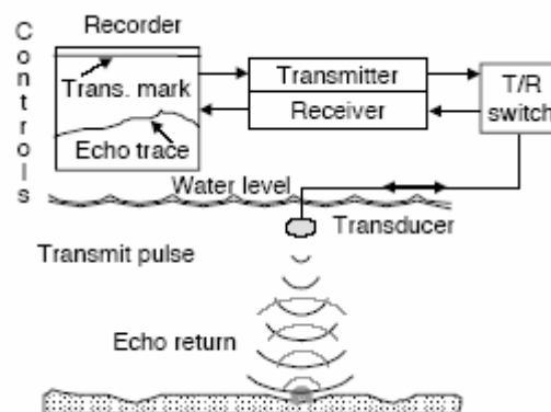
Figure 4.4. Basic echosounder operation
