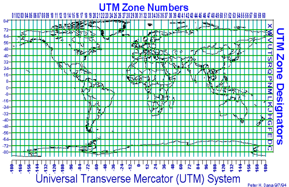
Figure 5.8. Universal transverse mercator (UTM) system
