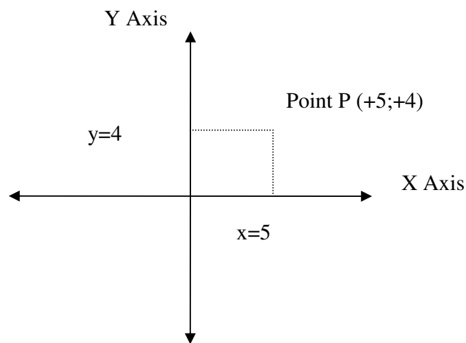
Figure 5.1. Cartesian coordinates in a plane
