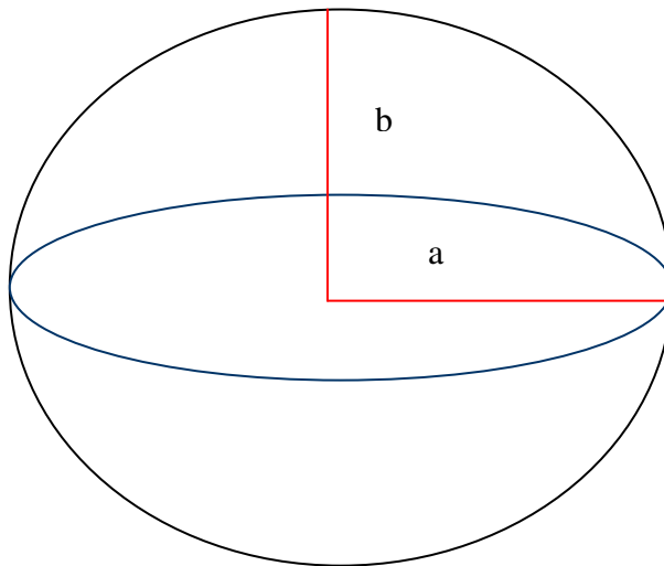
Figure 5.3. Ellipsoidal parameters
