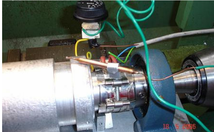
Figure 5.6: Heating Device mounted onto the third prototype
