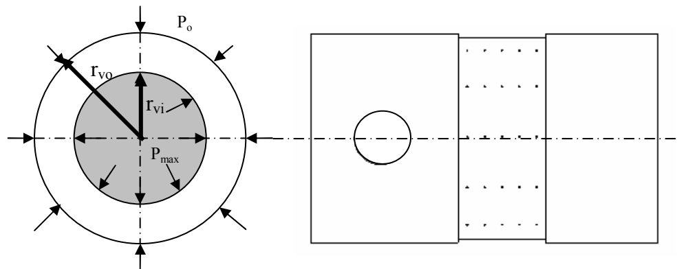
Figure 4.12: Illustration of inside and outside pressure for the vessel
