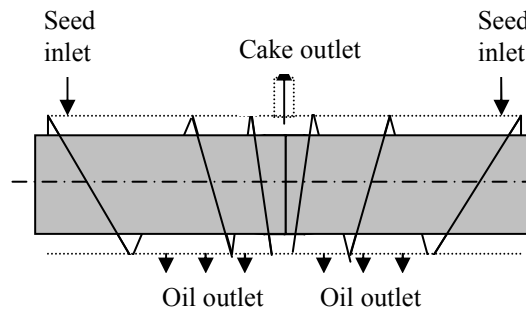
Figure 3.14: Illustration of the flow of the seeds in the first conceptual design
