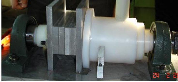
Figure 5.2: Second Prototype of Screw Press
