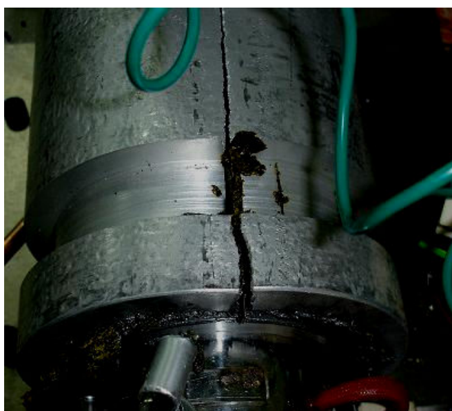
Figure 5.10: View of the failure on the vessel
