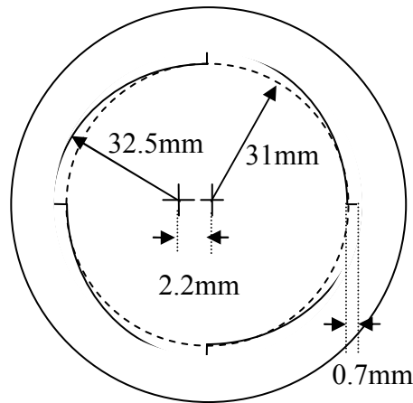
Figure 4.14: Illustration of the curvature shaped grooves and its dimensions
