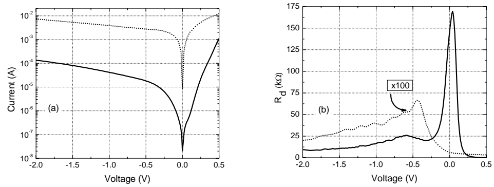
Figure 5.6: Current-voltage characteristics and differential resistance of 30 μm diameter photodetector at 300 K (dotted line) and 77 K (solid line).
