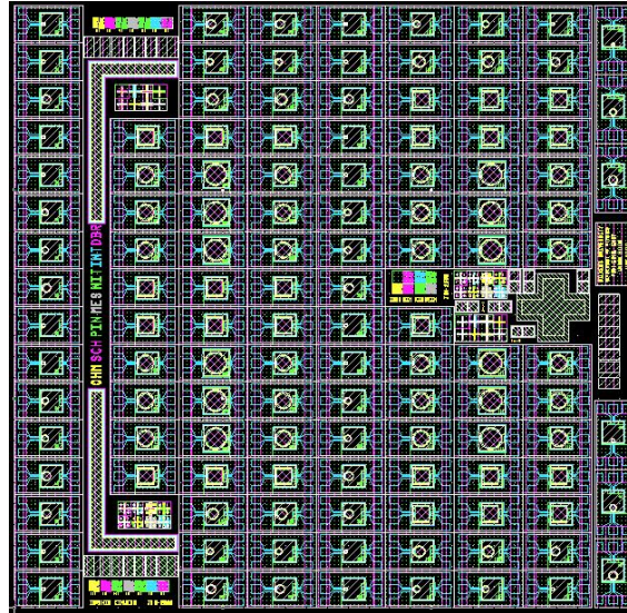
Figure 3.4: Plot of the mask containing large area photodetectors. All the fabrication steps are shown aligned to each other. The mask contains around 115 photodetectors.
