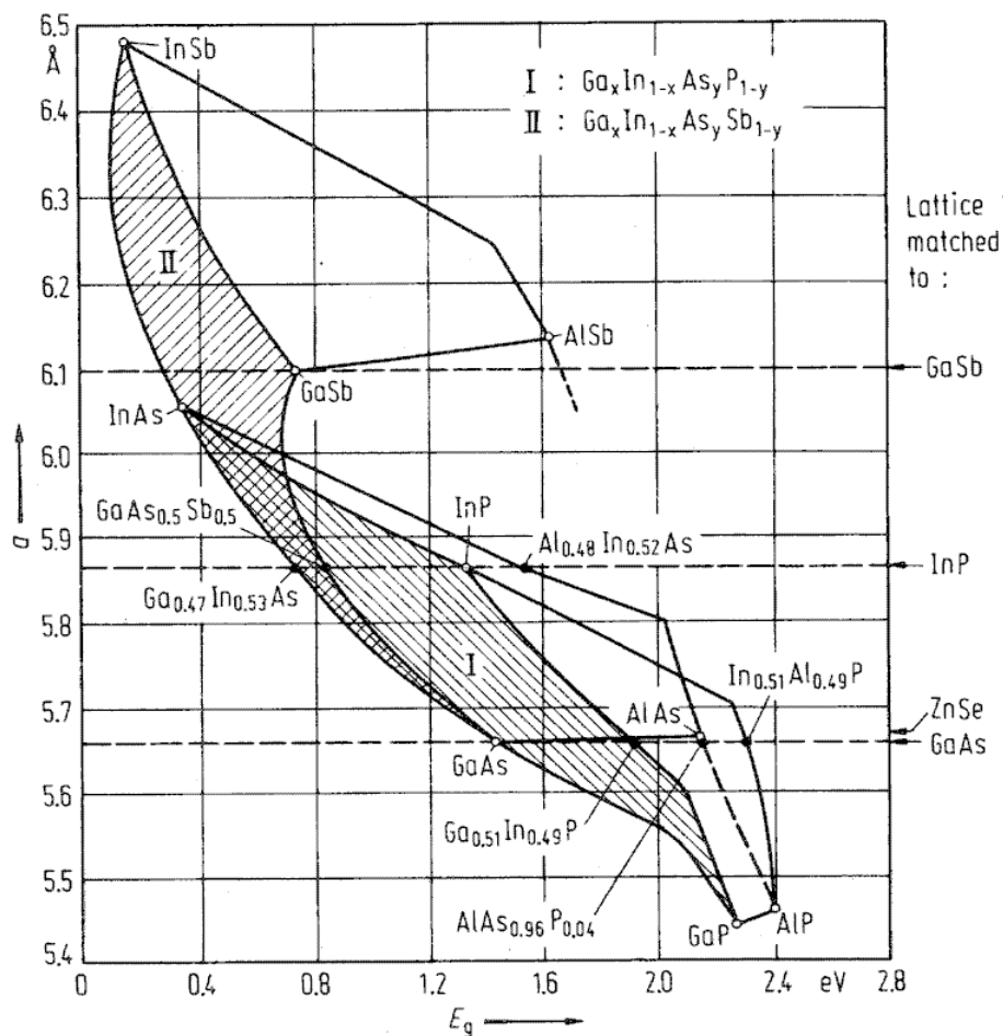
Figure 4.1: Lattice parameter vs. energy gap of III-V compounds used with InP and GaAs based devices (after reference [61]).
