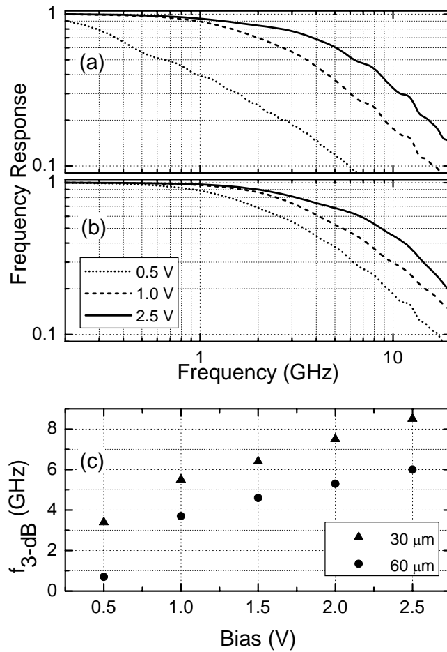
Figure 5.18: Fast Fourier Transform of the temporal responses of the photodetectors. Results for (a) 60 μm diameter and (b) 30 μm diameter photodetectors as a function of bias are shown. (c) 3-dB bandwidth of the 30 and 60 μm diameter photodetectors as a function of applied bias.
