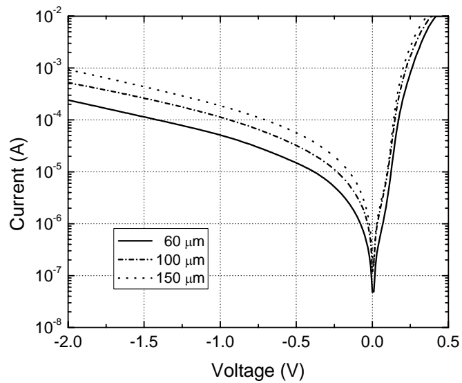
Figure 5.7: Measured current-voltage characteristics of 60, 100, and 150 μm diameter photodetectors at 77 K.
